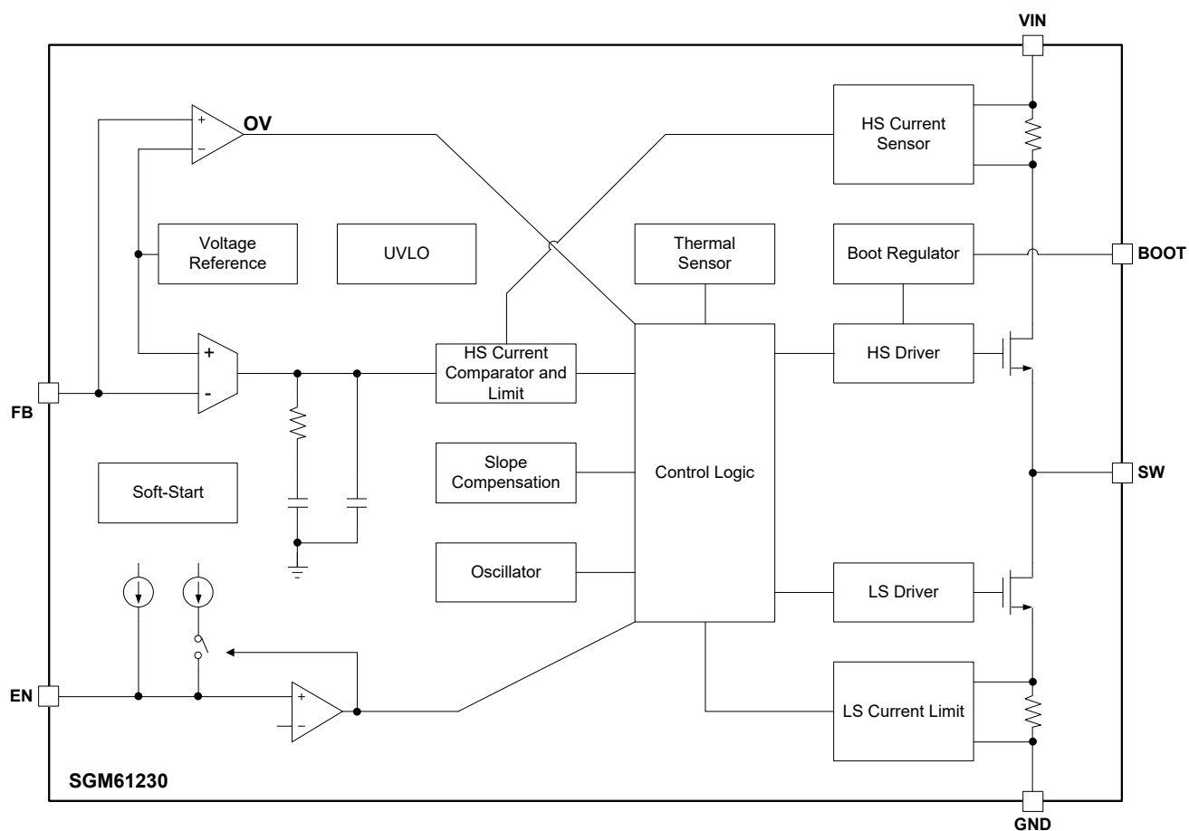
Figure 2. Block Diagram
