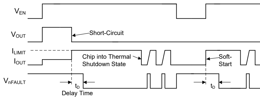
Figure 4. SGM2581A/C/E/G/I/K Fault Timing: Output Reset by Toggling EN
