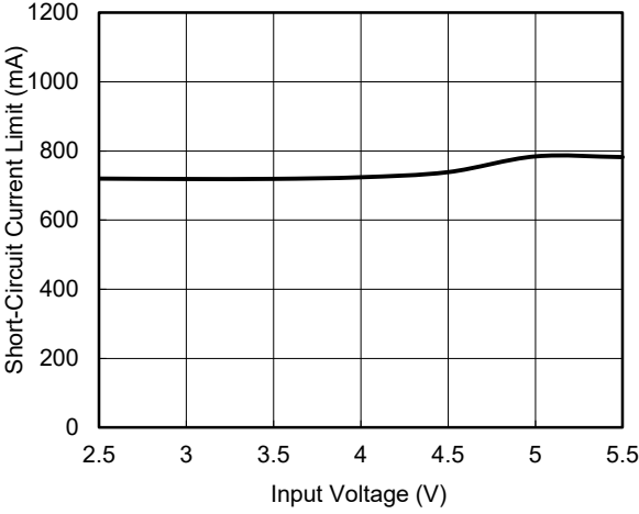
Short-Circuit Current Limit vs. Input Voltage (SGM2581A/B/G)
