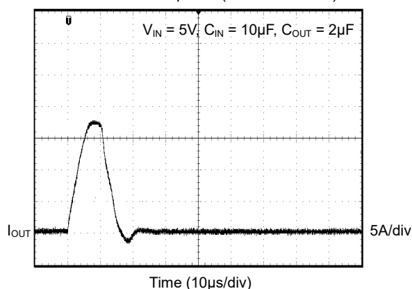
Short-Circuit Response (SGM2581A/B/G)
