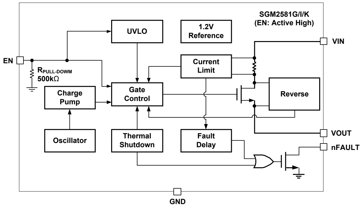
Figure 7. SGM2581G/I/K Block Diagram
