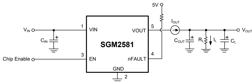
Figure 2. SGM2581 Test Circuit
