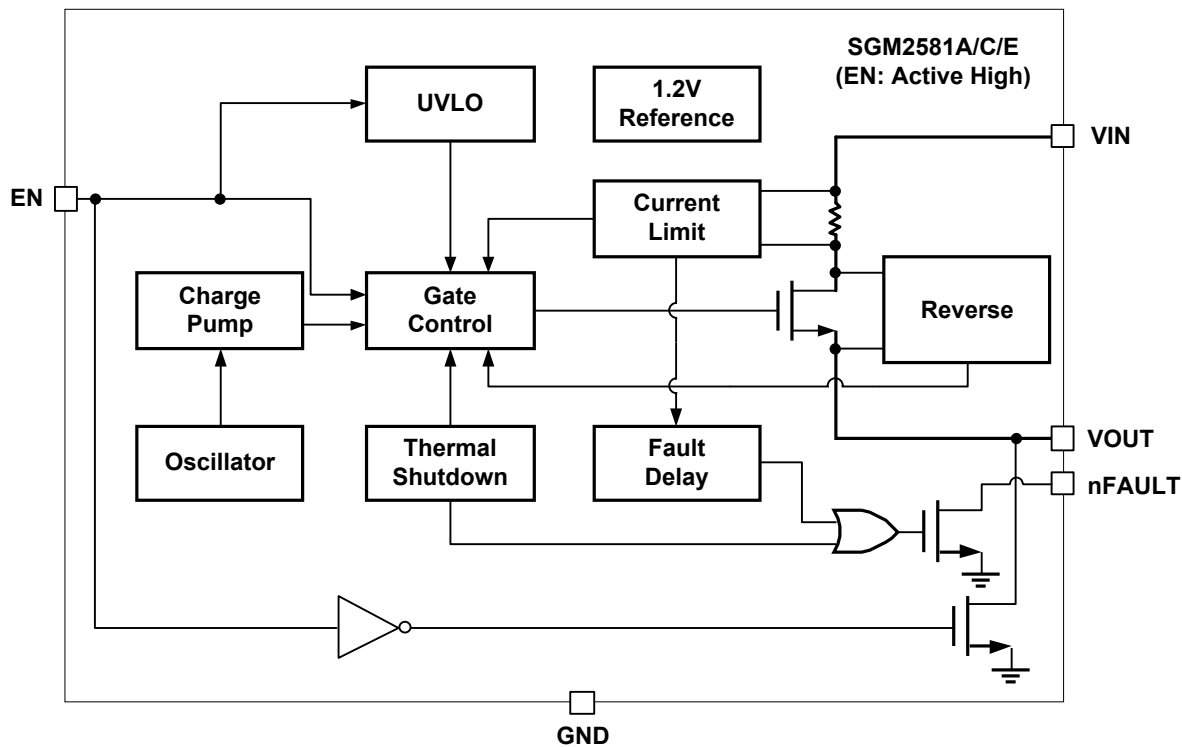
Figure 6. SGM2581A/C/E Block Diagram
