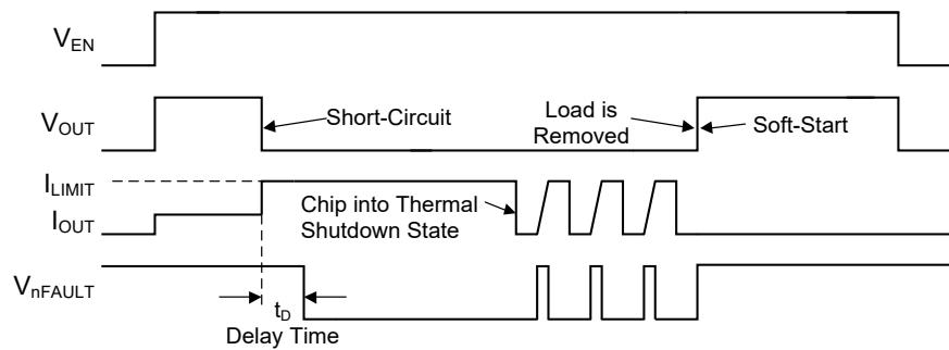
Figure 5. SGM2581A/C/E/G/I/K Fault Timing: Output Reset by Removing Load
