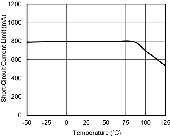
Short-Circuit Current Limit vs. Temperature (SGM2581A/B/G)
