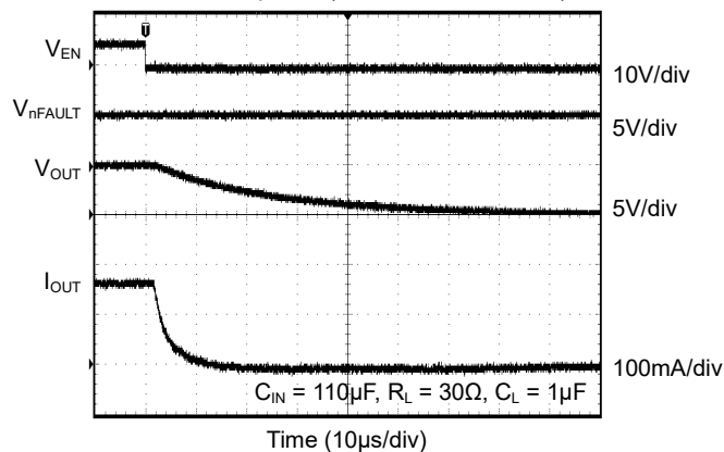
Turn-Off Response (SGM2581A/C/E/G/I/K)
