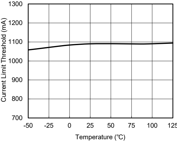
Current Limit Threshold vs. Temperature (SGM2581A/B/G)
