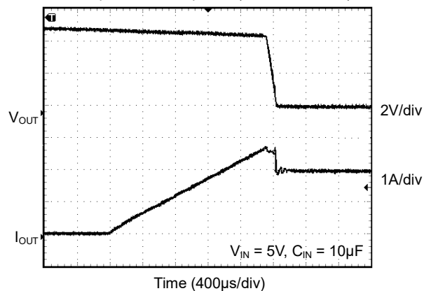
Ramped Load Response (SGM2581E/F/K)
