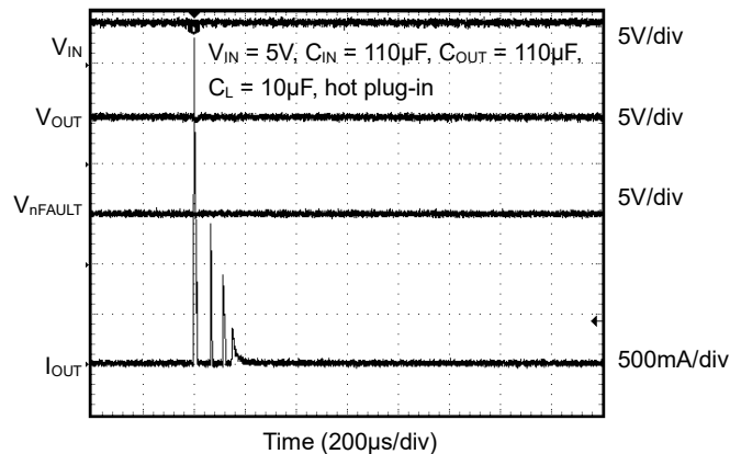
Capacitance Load Inrush Response (SGM2581A/B/G)
