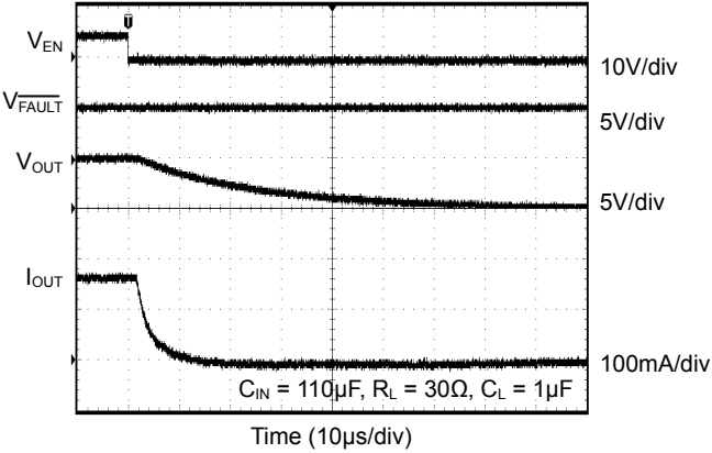
Turn-Off Response (SGM2581A/C/E/G/I/K)
