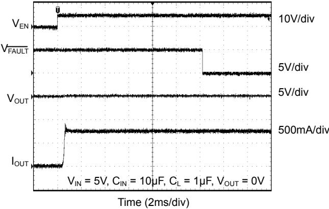
Enabled Into Short-Circuit (SGM2581A/G)
