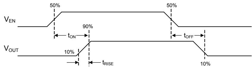
Figure 3. SGM2581A/C/E/G/I/K Switch Turn-On and Turn-Off Delay Times
