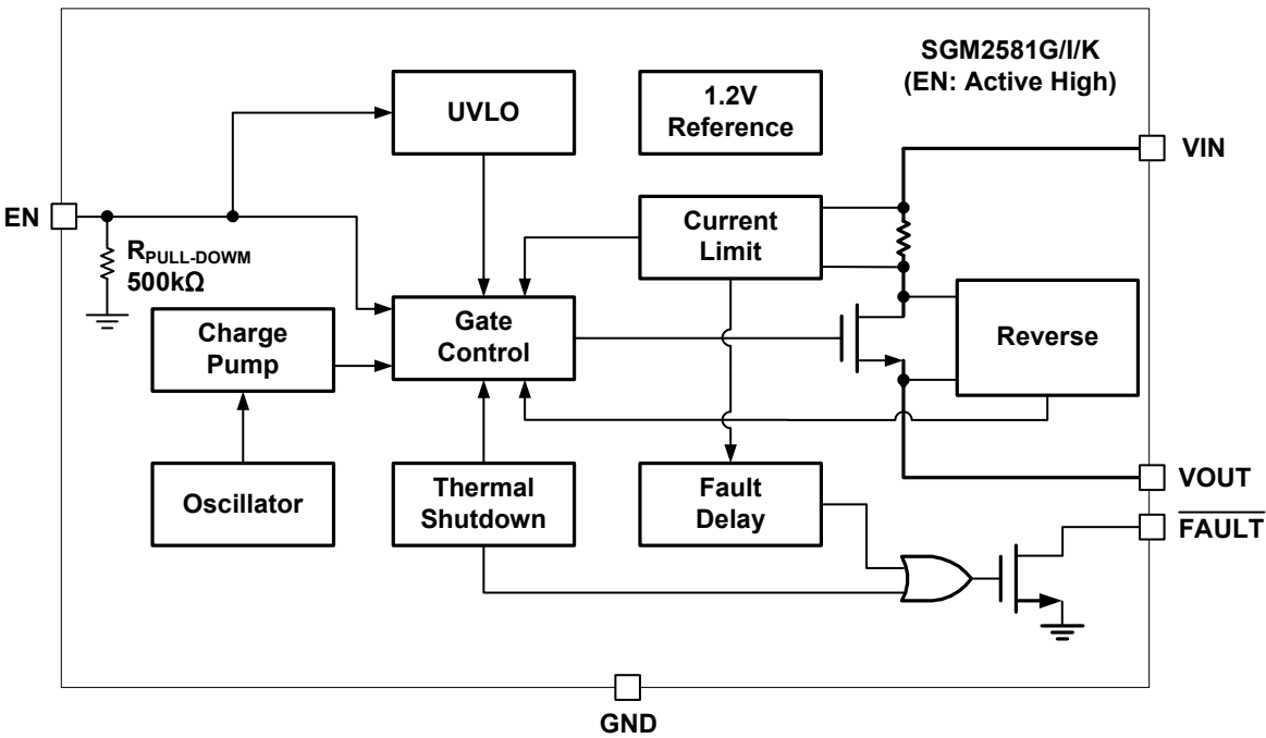
Figure 7. SGM2581G//K Block Diagram
