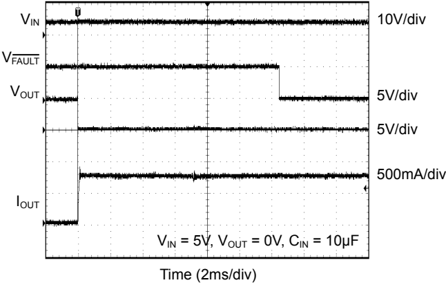
Short-Circuit Response (SGM2581A/B/G)
