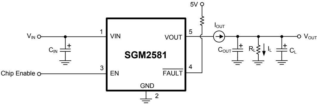
Figure 2. SGM2581 Test Circuit
