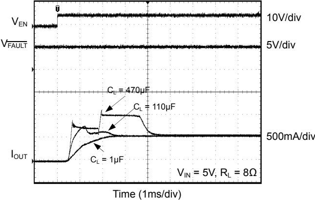
Inrush Current Response (SGM2581A/G)
