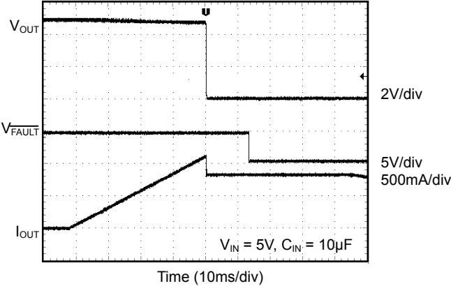
Ramped Load Response (SGM2581A/B/G)
