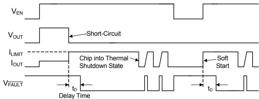
Figure 4. SGM2581A/C/E/G/I/K Fault Timing: Output Reset by Toggling EN
