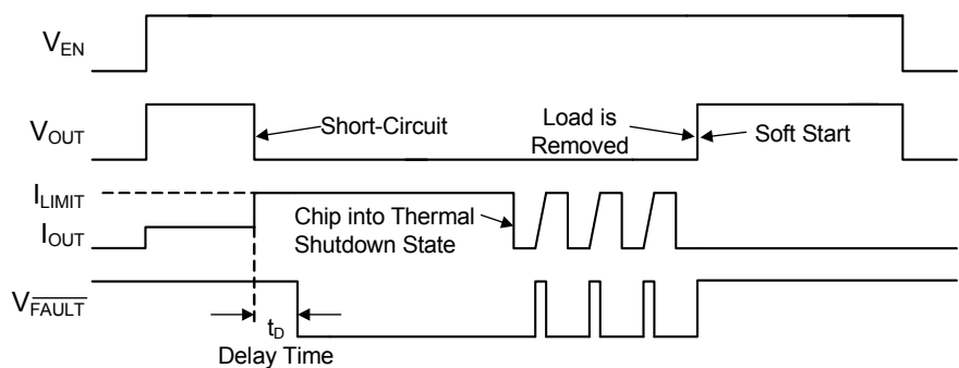
Figure 5. SGM2581A/C/E/G/I/K Fault Timing: Output Reset by Removing Load
