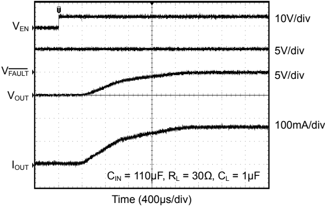
Turn-On Response (SGM2581A/C/E/G/I/K)
