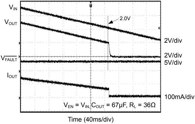
UVLO at V_{IN} Falling
