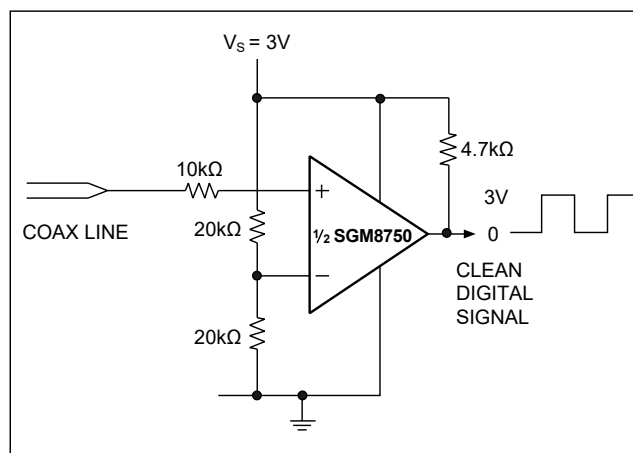
Figure 3. Line Receiver Application
