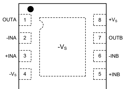
TDFN-2×2-8AL/TDFN-3×3-8BL
