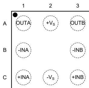
WLCSP-1.57×1.57-8B
