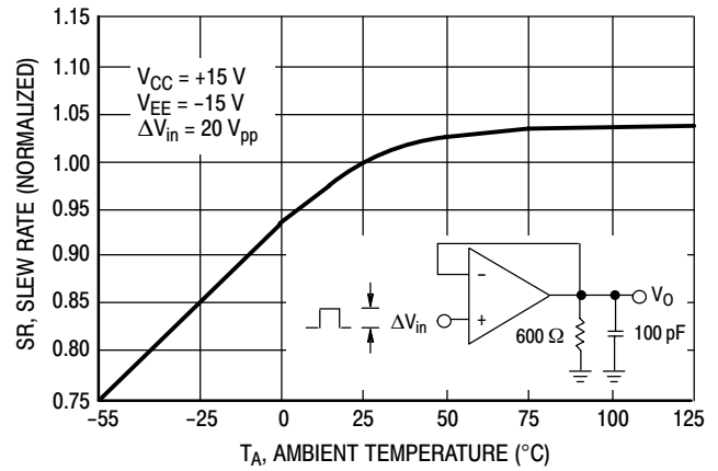
Figure 17. Normalized Slew Rate versus Temperature
