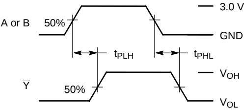
Figure 4. Switching Waveforms
