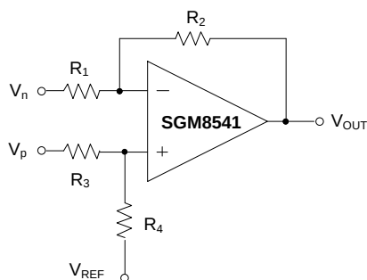
Figure 4. Differential Amplifier
