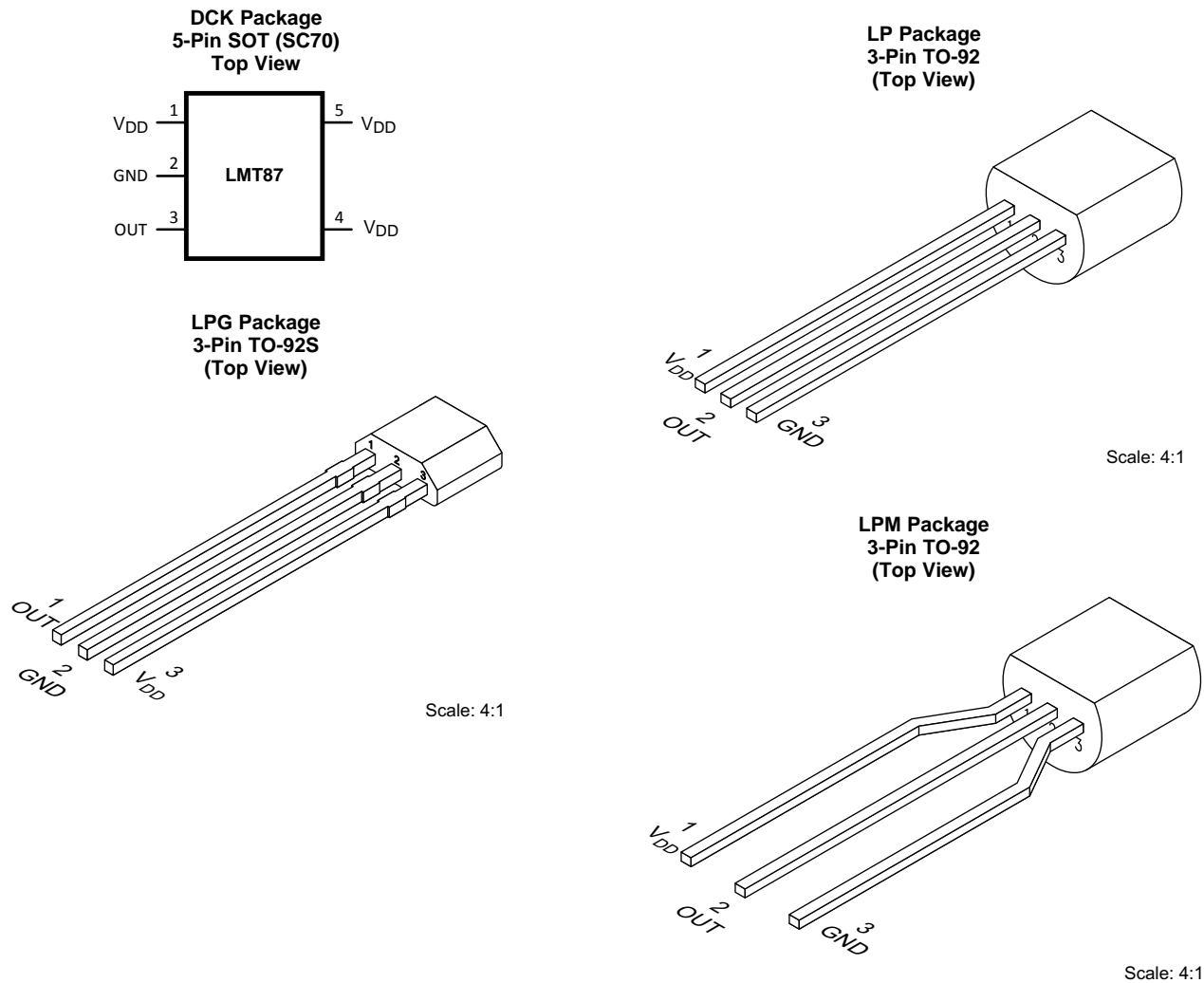
Pin Functions
