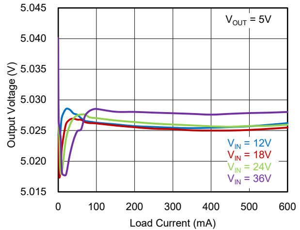
Load Regulation
