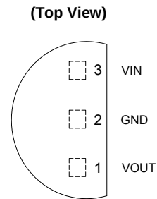
TO92 (Ammo Packing)
