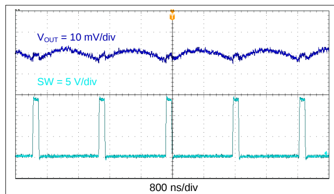
Figure 28. TPS563208 Output Voltage Ripple, I_{OUT} = 0 A
