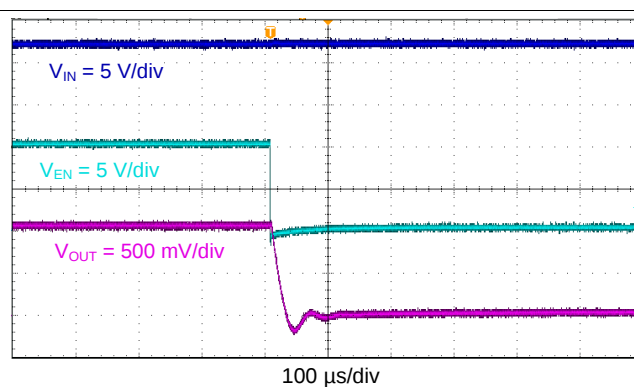
Figure 35. TPS563201 Shutdown Relative to EN
