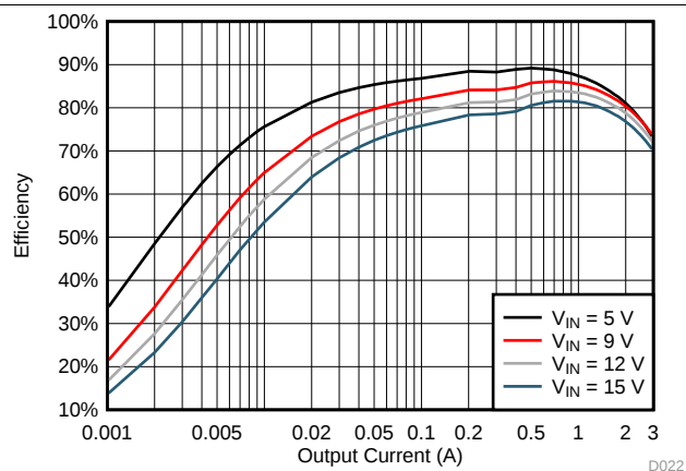
Figure 23. TPS563201 Efficiency
