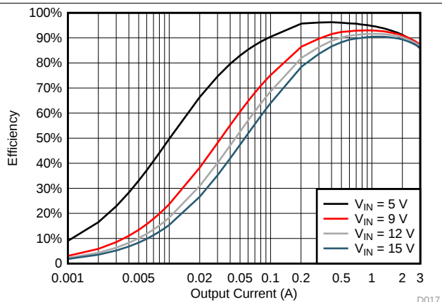
Figure 15. TPS563208 V_{OUT} = 1.5\text{ V} Efficiency, L = 2.2\text{ }\mu\text{H}
