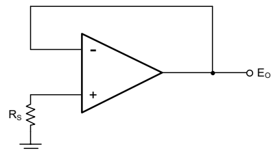
Figure 2. Unity-Gain Buffer Configuration
