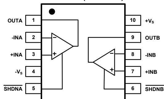
MSOP-10
