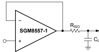
Figure 5. Capacitive-Load-Driving Circuit
