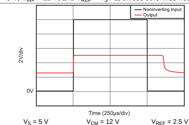
图 20. Noninverting Differential Input Overload
