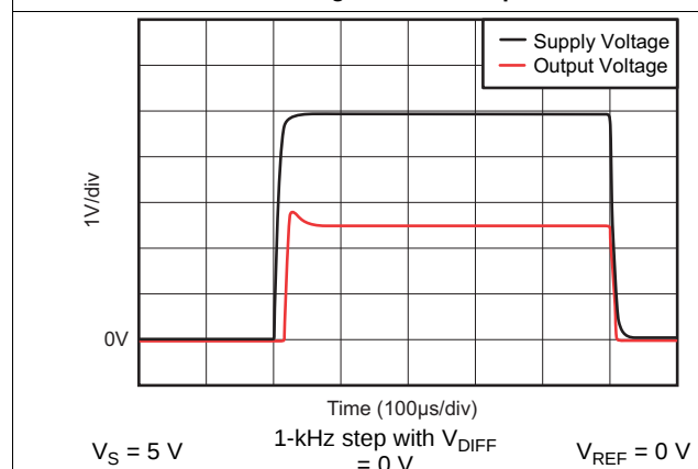
图 21. Start-Up Response
