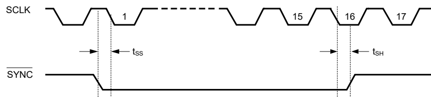
Figure 5. \overline{\text{SYNC}} Setup and Hold Times
