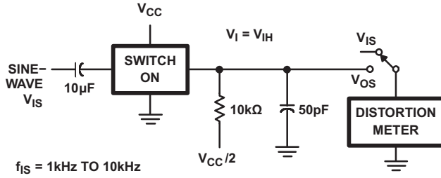
Figure 12. \frac{1}{4} Sine-Wave Distortion Test Circuit
