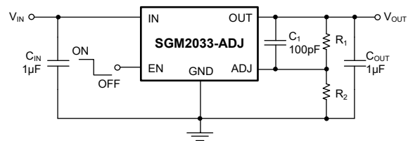
Figure 5. SGM2033-ADJ with External Resistor Divider
