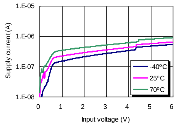
Detector threshold=4.4V
