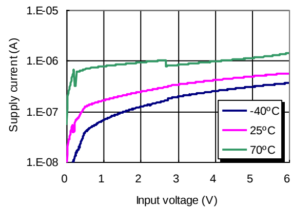
Detector threshold=2.7V
