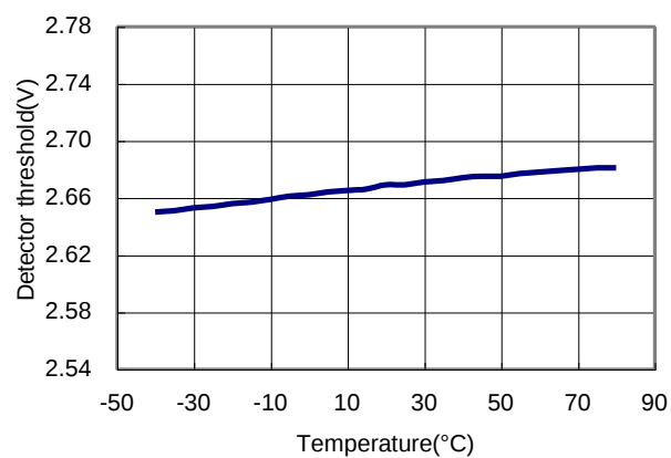
Detector threshold=2.7V
