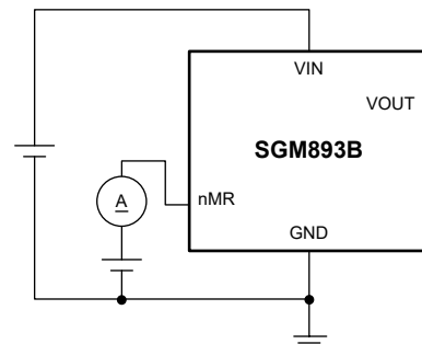
Test Circuit 6
