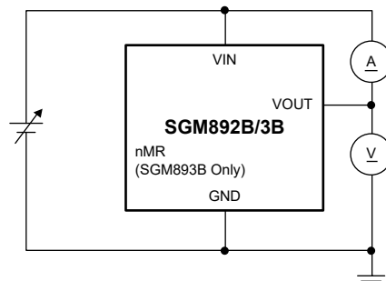
Test Circuit 4
