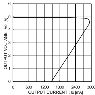
Fig.5 Load Regulation
