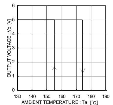
Fig.12 Thermal Shutdown Circuit Characteristics
