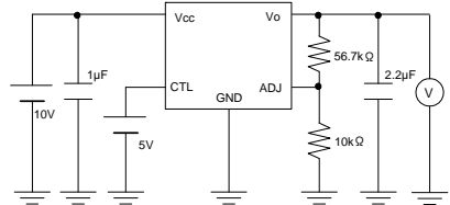
Measurement Circuit of Fig.8
