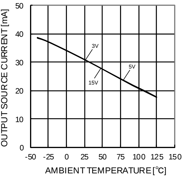
Figure 56. Output Source Current - Ambient Temperature (OUT=0V)
