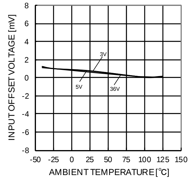
Figure 62. Input Offset Voltage - Ambient Temperature ( V_{ICM}=0V , OUT=1.4V )
