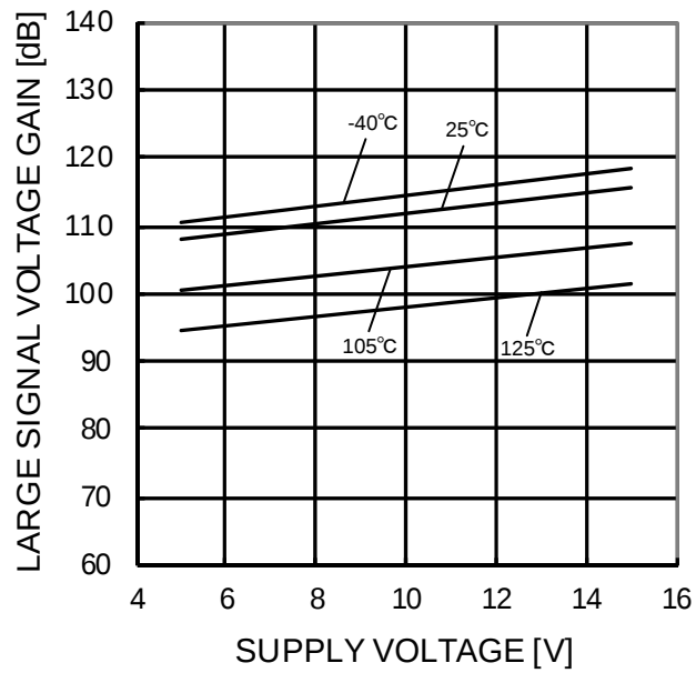
Figure 69. Large Signal Voltage Gain - Supply Voltage (R L =2kΩ)
