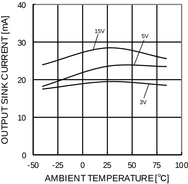
Figure 34. Output Sink Current - Ambient Temperature (OUT=VCC)
