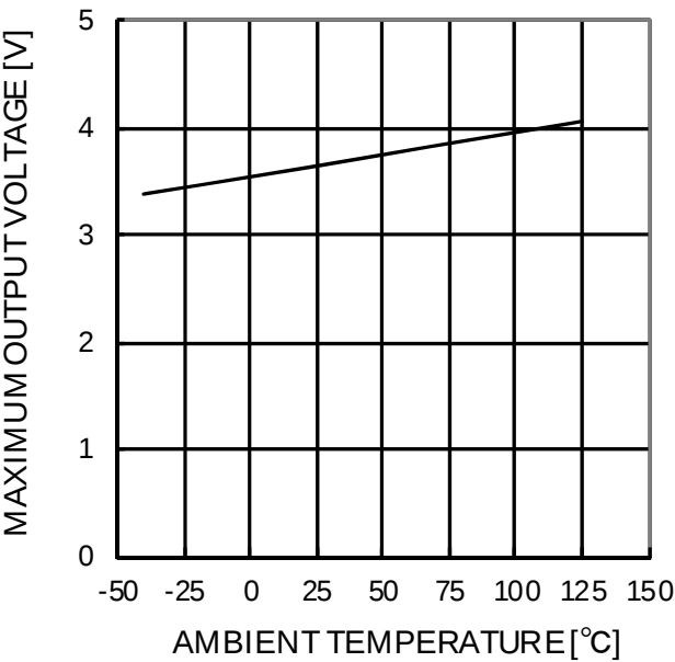
Figure 54. Maximum Output Voltage - Ambient Temperature (VCC=5V, RL=2kΩ)
