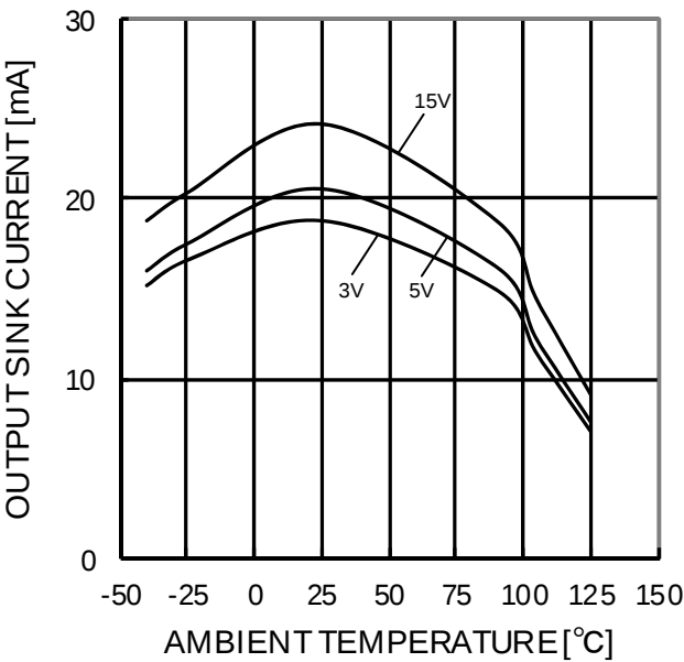
Figure 82. Output Sink Current - Ambient Temperature (OUT=VCC)
