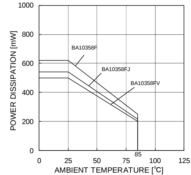
Figure 2. Derating Curve
