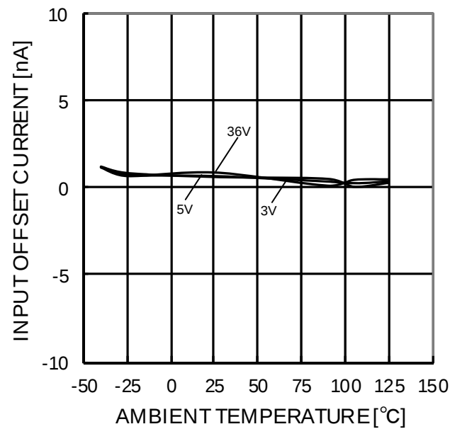
Figure 68. Input Offset Current - Ambient Temperature (V ICM =0V, OUT=1.4V)
