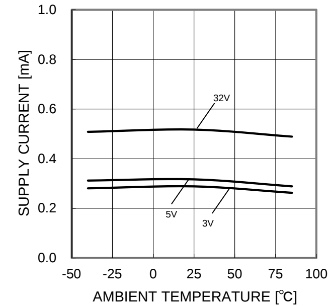
Figure 4. Supply Current – Ambient Temperature
