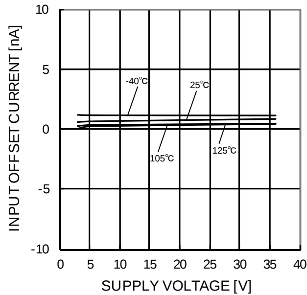
Figure 67. Input Offset Current - Supply Voltage (V ICM =0V, OUT=1.4V)
