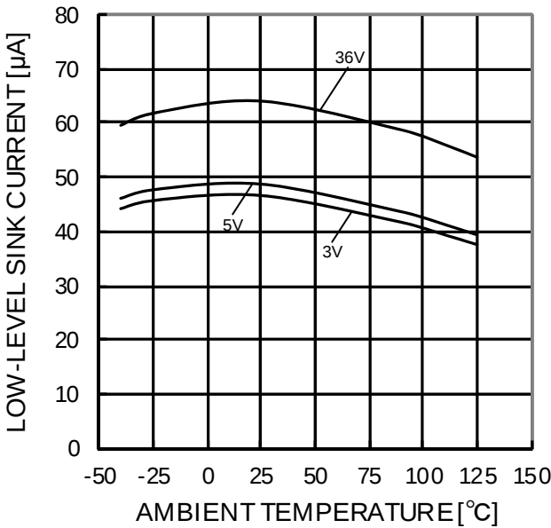
Figure 84. Low Level Sink Current - Ambient Temperature (OUT=0.2V)
