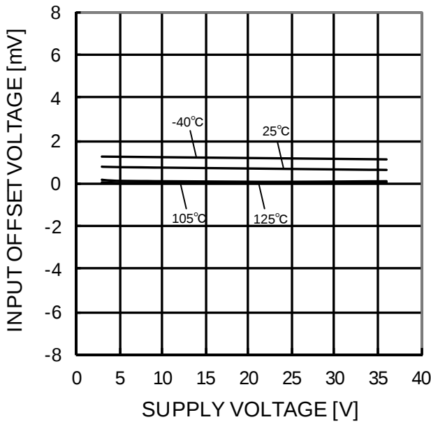
Figure 85. Input Offset Voltage - Supply Voltage (V ICM =0V, OUT=1.4V)
