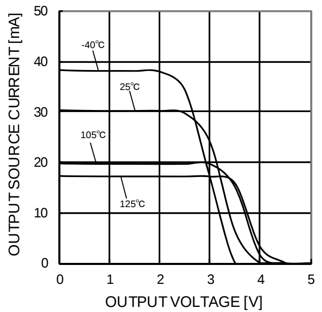
Figure 79. Output Source Current - Output Voltage (VCC=5V)
