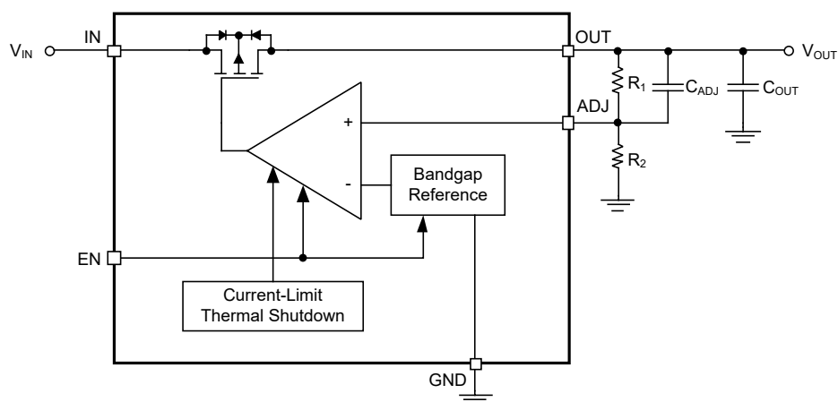
Figure 5. Low Noise Adjustable Regulator (SOIC-8, TDFN-3×3-8L and TO-263-5B Versions)
