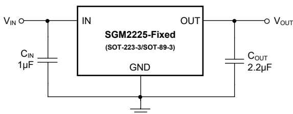
Figure 1. Fixed Voltage Typical Application Circuit
