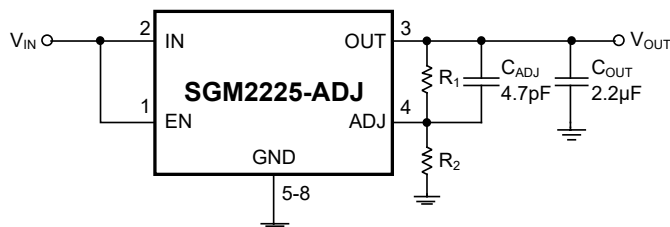
Figure 7. Low Noise Adjustable Output Voltage Application
