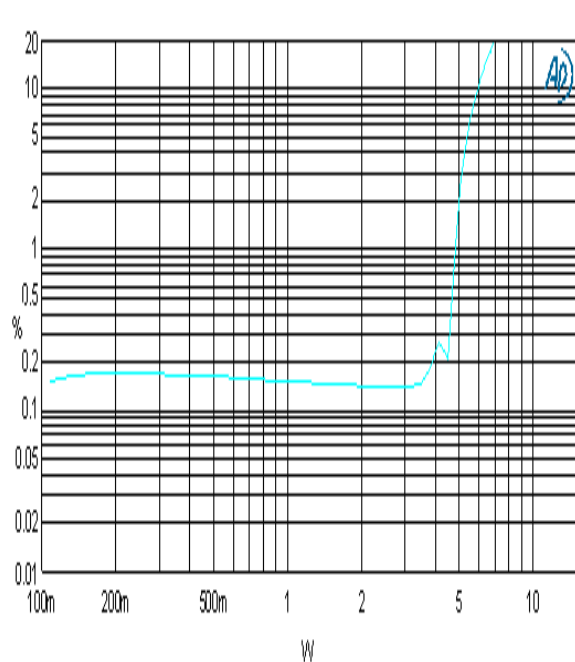
THDN_PO@9V 4OHM
