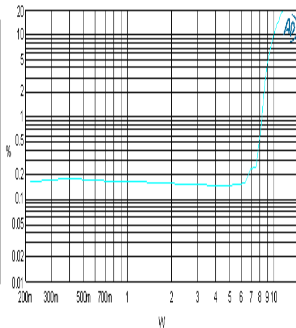
THDN_PO@12V 8OHM
