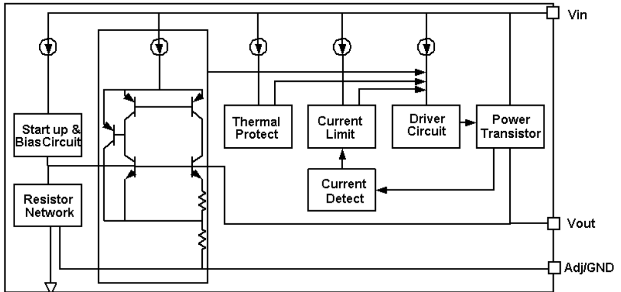
Fig 3. Block Diagram
