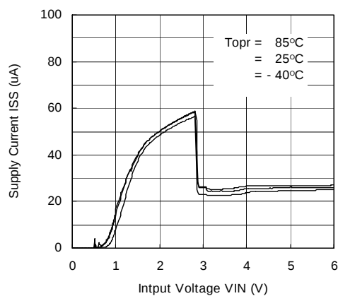
XC6401(2.85V)
