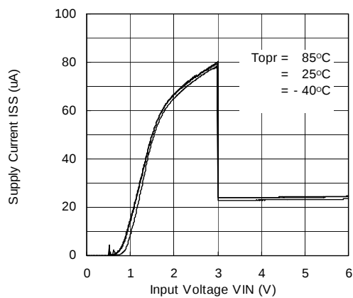
XC6401(3.0V)
