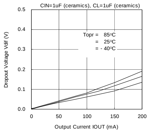
XC6401(5.0V)
