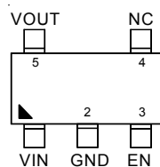
SOT-23-5 (R-Type)
