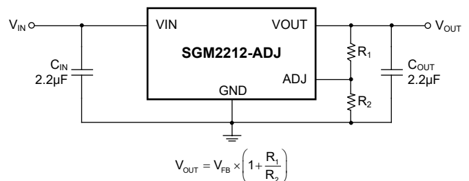
Adjustable Voltage Typical Application Circuit
