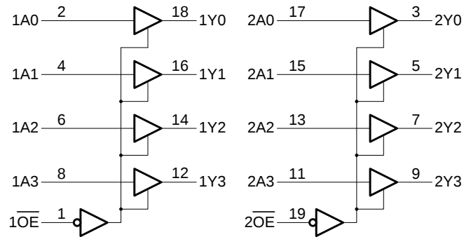
Figure 1. Logic symbol
