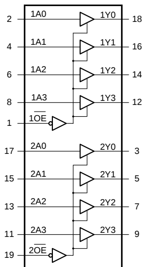
Figure 3. Functional diagram
