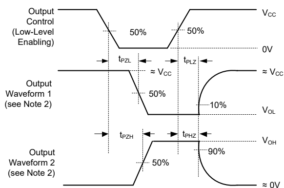
Voltage Waveforms Enable and Disable Times for 3-State Outputs
