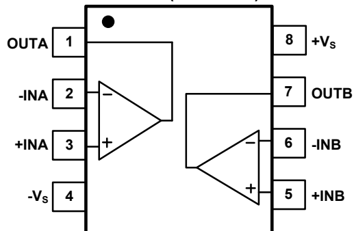
SGM722 (TOP VIEW)
